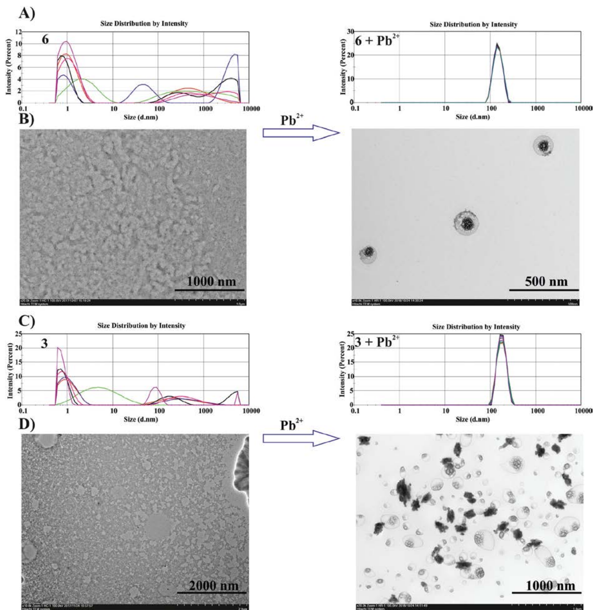
Fig. 5 (A) Left: Size distribution of the particles by intensity from a solution of macrocycle 6 ( 1 \times 10^{-4} M), right: size distribution of the particles by intensity from a solution of macrocycle 6 ( 1 \times 10^{-4} M) and Pb(NO_3)_2 ( 1 \times 10^{-4} M) at a molar ratio of 1 : 1 in chloroform. (B) Left: TEM images of macrocycle 6, right: TEM images of the aggregates formed by macrocycle 6 and Pb(NO_3)_2 . (C) Left: Size distribution of the particles by intensity from a solution of macrocycle 3 ( 1 \times 10^{-4} M) and Pb(NO_3)_2 ( 1 \times 10^{-4} M) at a molar ratio of 1 : 1 in chloroform. (D) Left: TEM images of macrocycle 3, right: TEM images of the aggregates formed by macrocycle 3 and Pb(NO_3)_2 .
