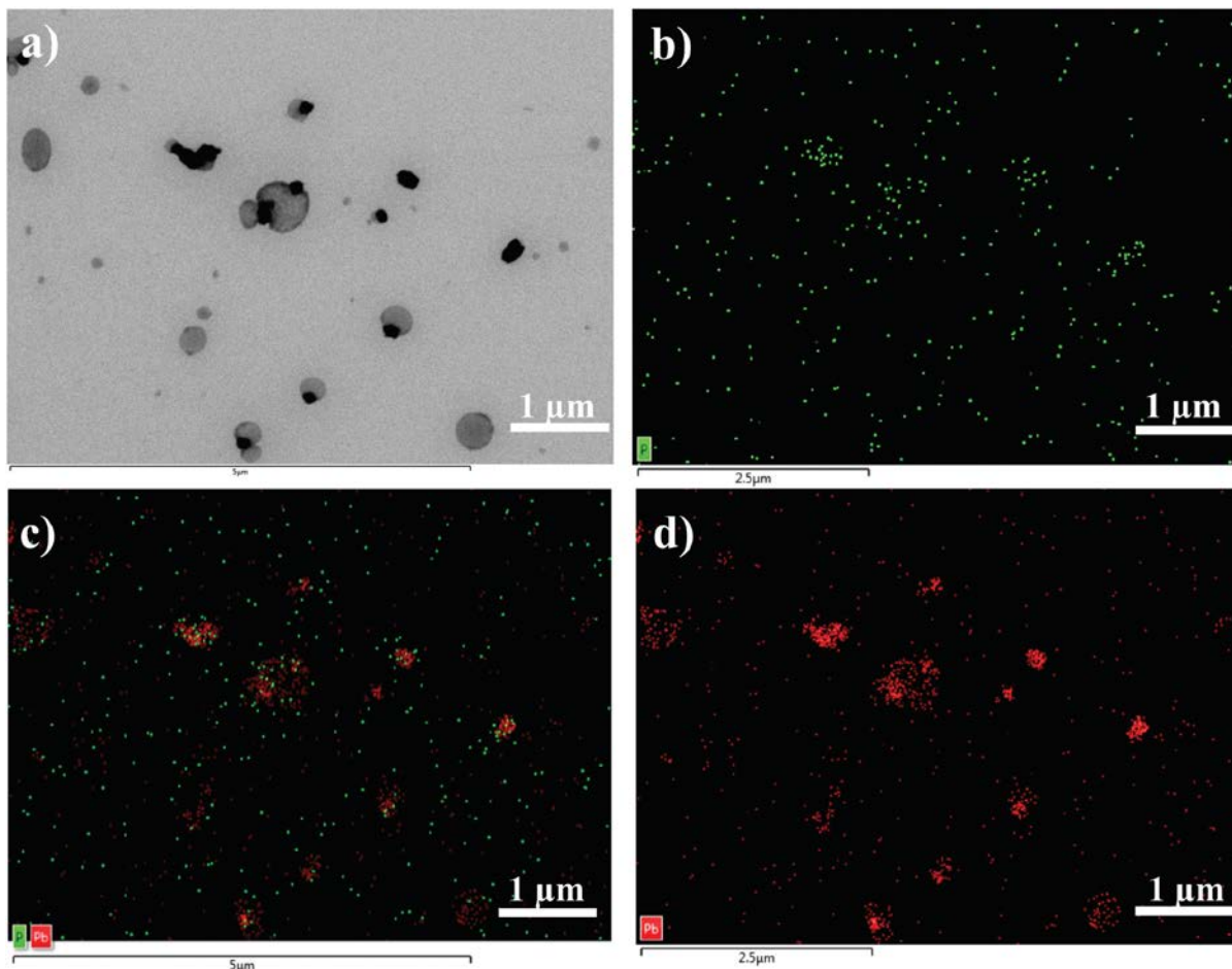
Energy-dispersion spectra of fractal structures formed by pillar[5]arene 6 and Pb_{2+} on a copper support. (A) Supramolecular nanometer-sized aggregates formed by compound 6 and Pb_{2+} ; (B) mapping of P; (C) superposition of elemental maps of P and Pb in the spherical aggregates formed by pillar[5]arene 6 and Pb_{2+} ; (D) mapping of Pb_{2+} .
