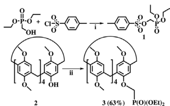
Scheme 1 Reagents and reaction conditions: (i) \text{NEt}_3/(\text{CH}_3\text{CH}_2)_2\text{O} , (ii) 1, \text{Cs}_2\text{CO}_3/\text{CH}_3\text{CN} .
