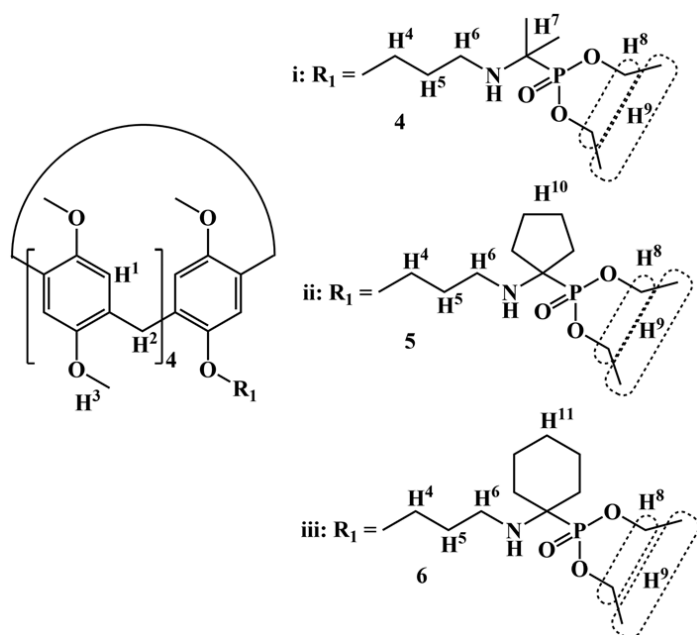
Fig. 2 Monosubstituted pillar[5]arenes containing the 1-aminophosphonate fragment.
