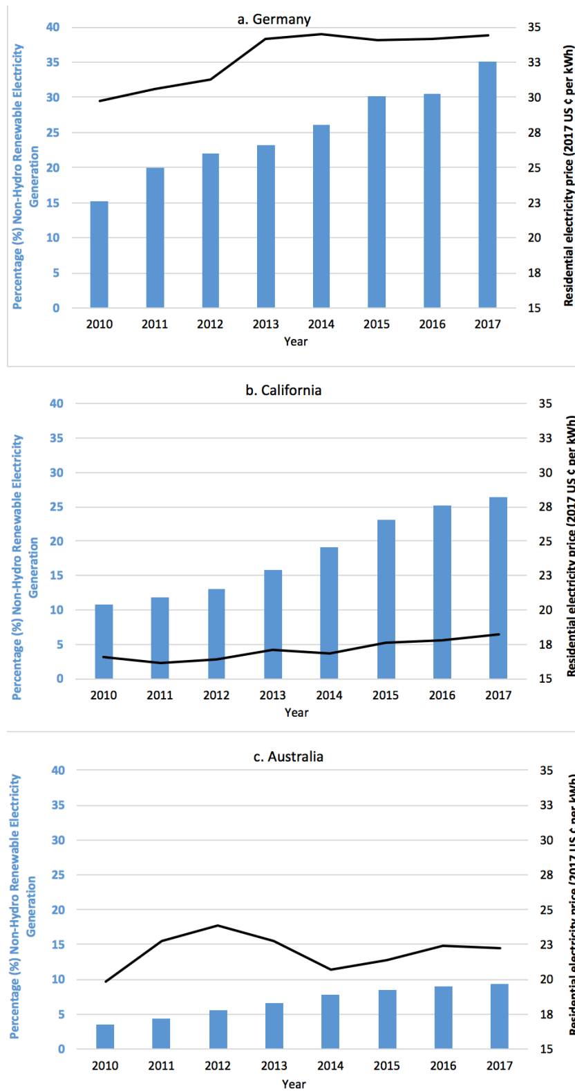
Figure 1: Non-hydro renewable electricity penetration (blue bars) and residential electricity prices (black lines) in 2010-2017. Sources: (1,23,35,36,37,38,39).
