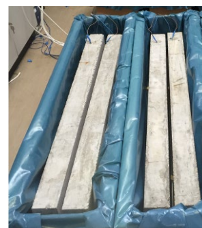
Figure 2. Accelerated corrosion setup
