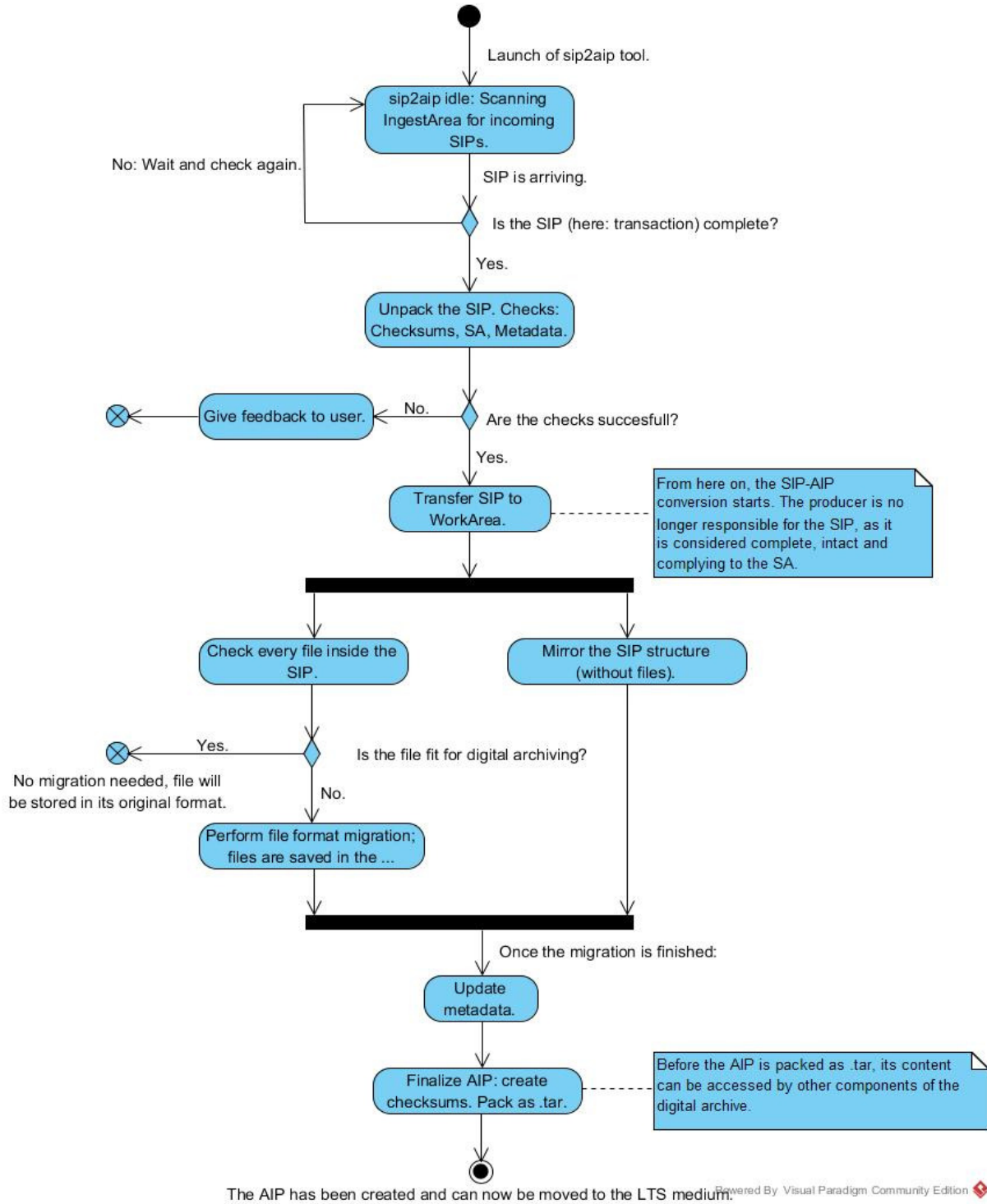
Figure 8: SIP2AIP Overview
