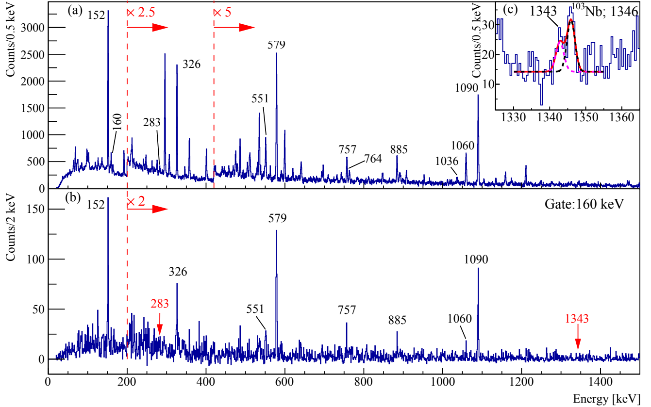
FIG. 3. (Color online) The \gamma -ray energy spectrum measured by EURICA in coincidence with a position-correlated \beta -decay occurring within 1.5 s of an implanted ^{102}\text{Y} ion. The labeled energies are those that correspond to transitions that are in the decay cascade originating from the 4^- isomeric state. The other energy peaks are due to the decay of levels populated in the \beta -decay of ^{102}\text{Y} which are independent of the cascade from the 4^- state and the random correlations of \beta -decays to nuclei other than ^{102}\text{Y} . The magnification factors shown in red are always given with respect to the original spectrum. (b) The spectrum measured in prompt ( \Delta T < 200 ns) coincidence with the 160-keV transition. The red labels in (b) indicate the positions of the 283- and 1343-keV transitions. (c) Is an expanded view of the region around the 1343-keV transition showing the result of a double-Gauss fit on a constant background, see text for details.
