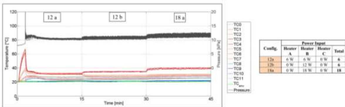
Figure 6. Test performed providing to the device 18 W solely at the heater B.
