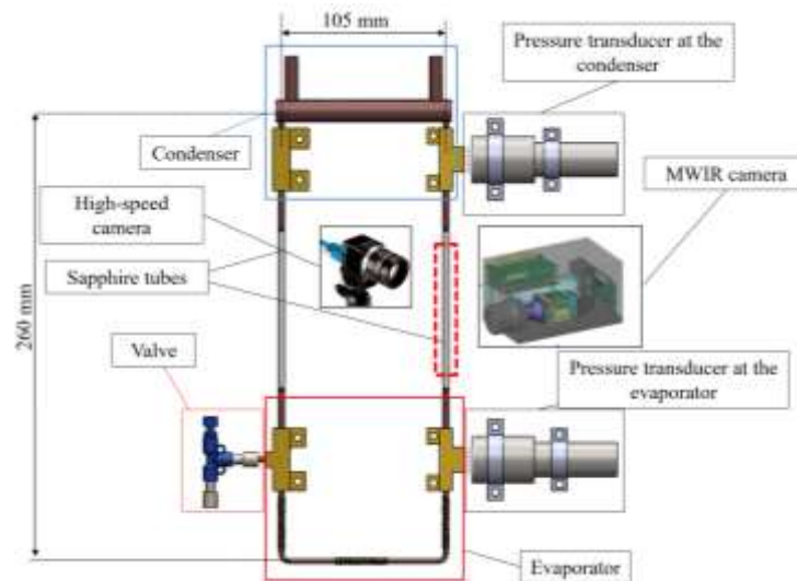
Figure 1. Main components of the SLPHP and thermocouples position. It is pointed out, with a dashed red rectangular contour, the sapphire section in which both high speed visualization and IR analysis are performed.
