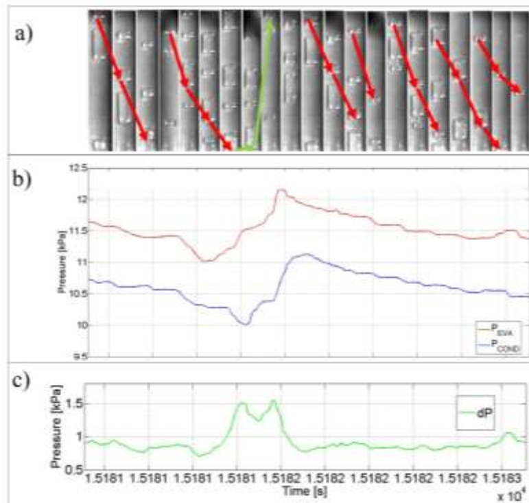
Figure 7. Flow visualization and pressure drop between a) the images obtained in the transparent section; b) pressure measurements at the evaporator (red line) and at the condenser (blue line). In c) the pressure drop measurements.
