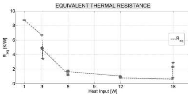
Figure 5. Equivalent thermal resistance for all the heating distribution tested
