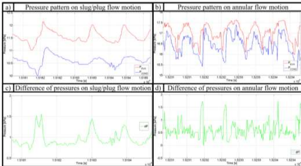
Figure 8. a) Pressure recorded in the heated (red line) and in the cooled region (blue line) in the case of a) slug/plug flow and b) annular flow. Pressure drop measurements (green line) in the case of c) slug/plug flow and d) annular flow.
