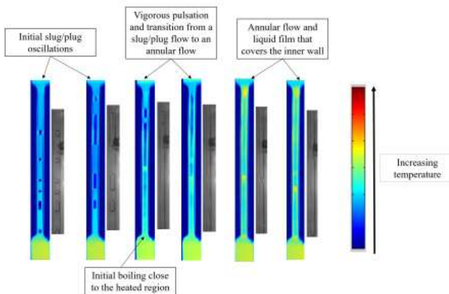
Figure 11. More relevant events observed during the start-up providing to the device a local heating power of 6 W just below the sapphire insert.
