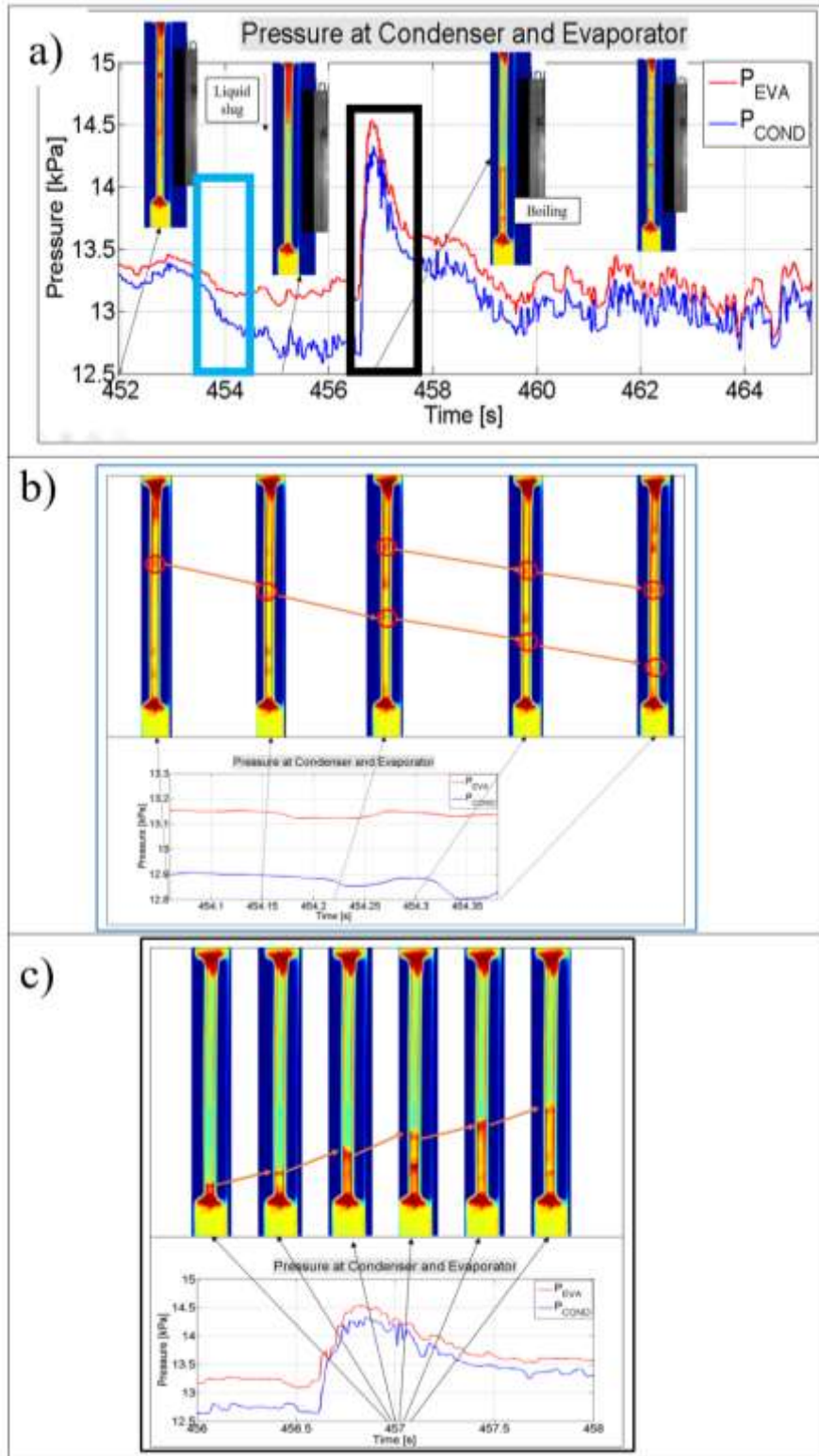
Figure 12. a) Synchronized pressure signals and IR images when the flow is oscillating in the loop. b) Zoom of the blue rectangular shape in a); c) Zoom of the black rectangular shape in a).
