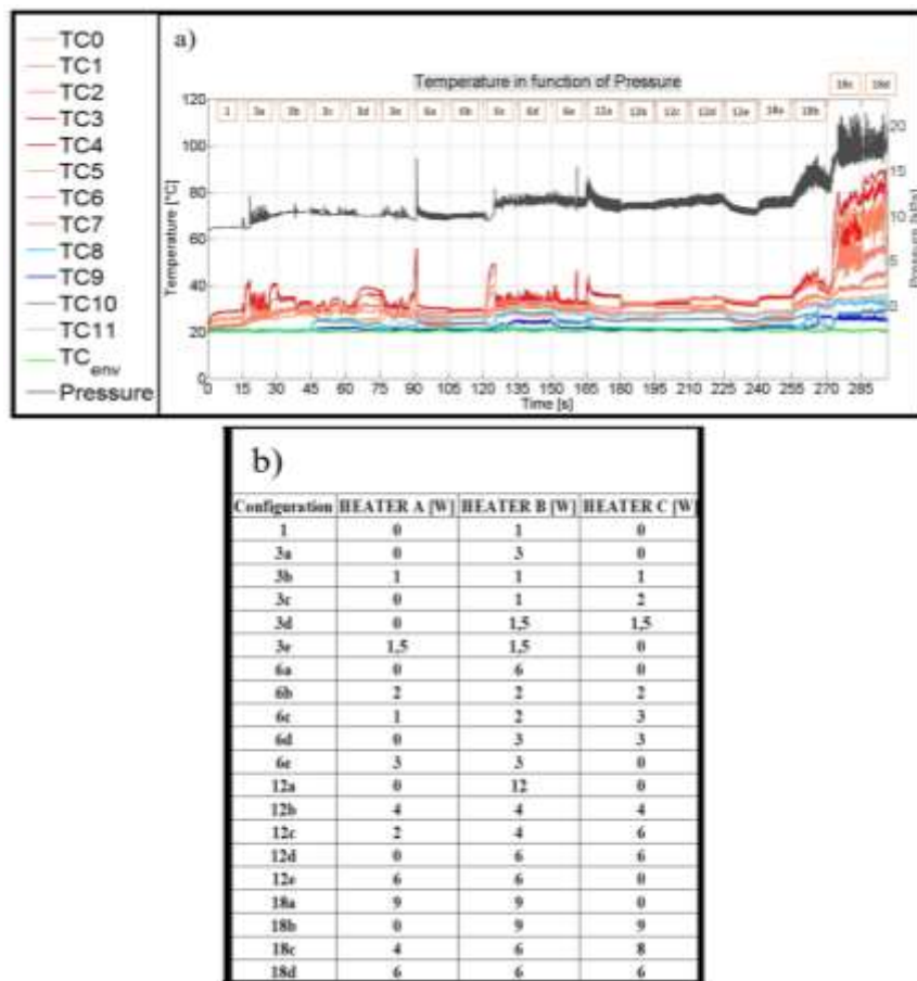
Figure 3. A) Temperatures and pressure evolution during the long-time test; B) the heating configurations tested.
