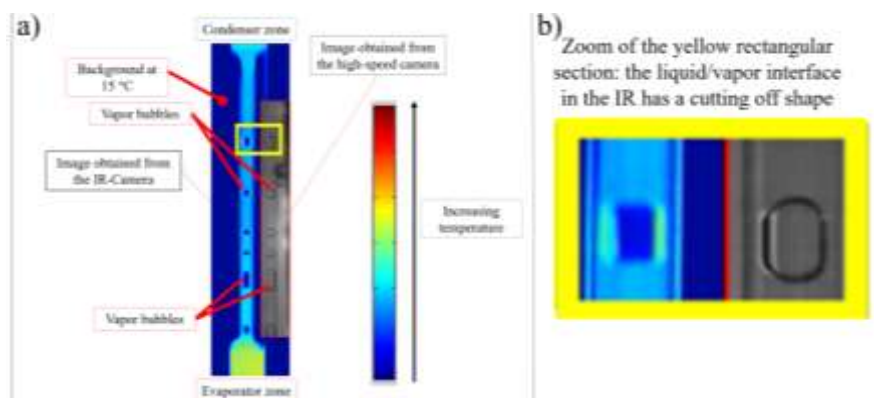
Figure 10. a) Slug-plug image obtained from the IR and the high-speed visualization; b) Zoom of the yellow section.
