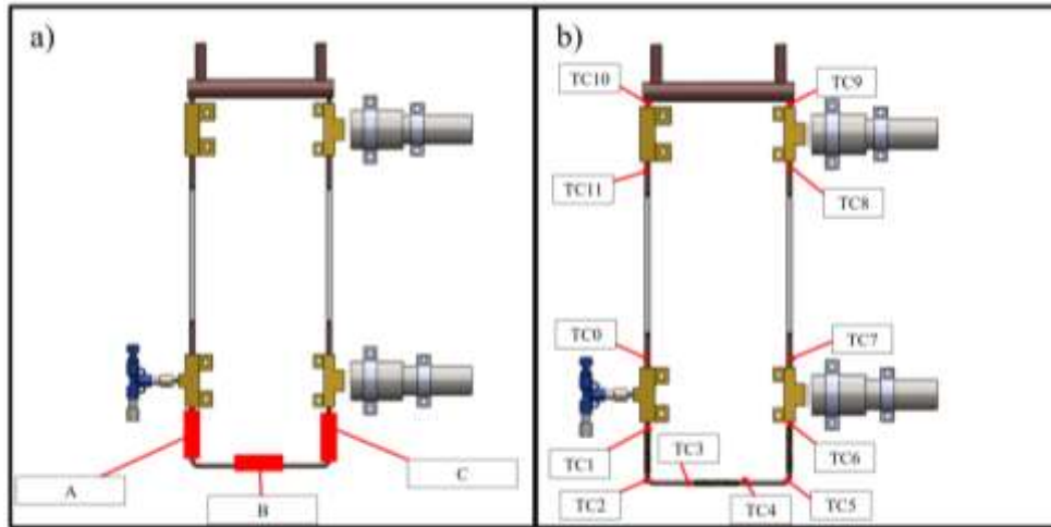
Figure 2. a) Heating element position; b) Thermocouple positions
