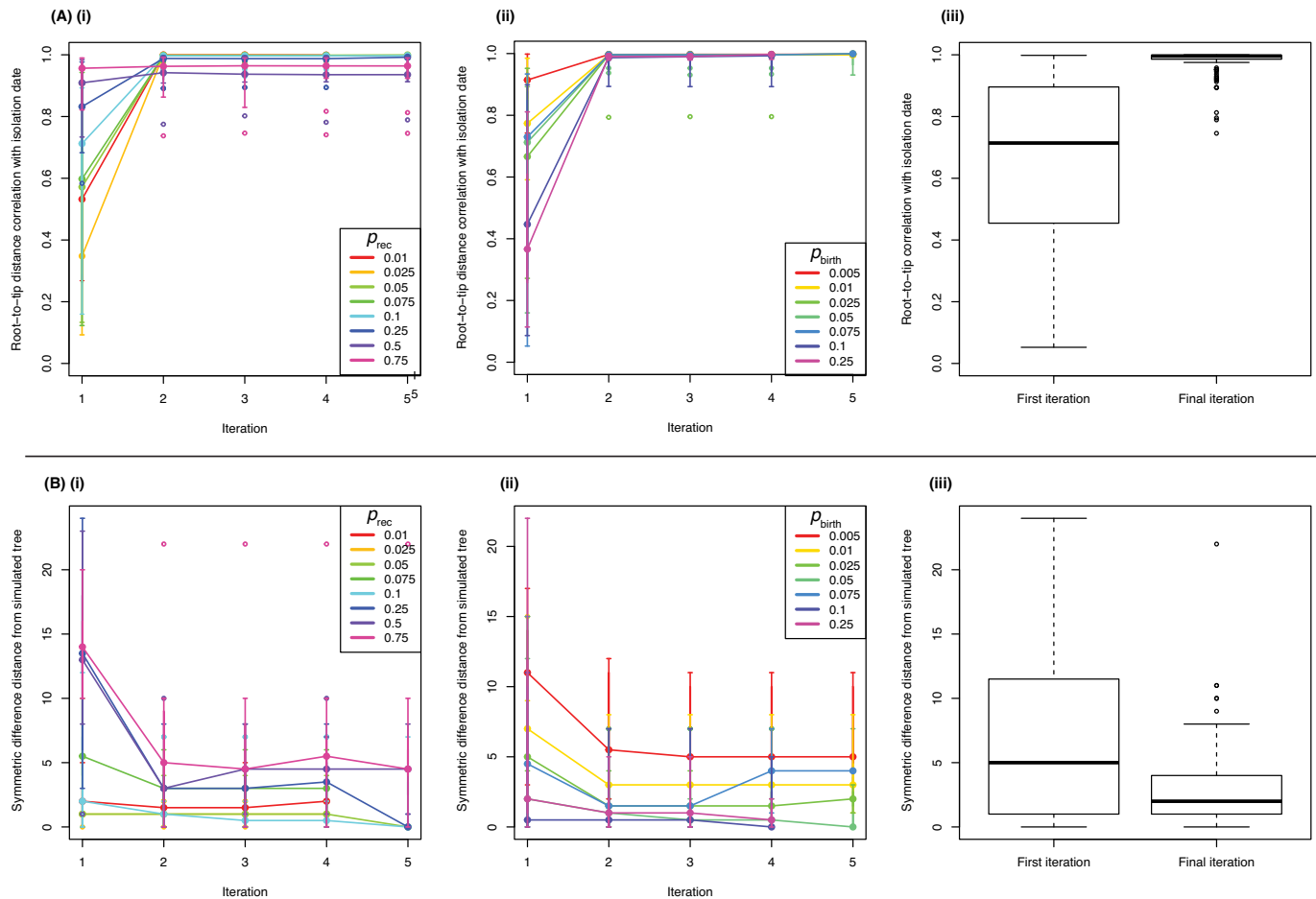
Figure 2. Accuracy of phylogenetic reconstructions from Gubbins analyses. (A) Accuracy of branch length estimation. (i) For each simulated dataset represented in Figure 1A, the Pearson correlation ( R^2 ) of the root-to-tip distances of simulated sequences with the number of time steps over which they had been diverging from the original sequence was calculated for the phylogenies from each iteration of the Gubbins analyses. The solid points linked by lines represent the median of the 10 simulations for each parameter set at each iteration; the vertical bars indicate the most extreme datapoints within 150% of the interquartile range. Empty circled points indicate outliers beyond this boundary. The color of each line indicates the p_{rec} parameter value in the simulations. (ii) The same statistics were calculated for the simulations displayed in Figure 1B. The results are displayed as in panel (i), with the color of the line representing the p_{birth} parameter value used in the simulation. (iii) Box and whisker plot summary of the R^2 values for all simulations represented in Figure 1 for the 'naïve' phylogenies in the first iteration and the phylogenies from the final iteration. The whiskers extend to the most extreme datapoints within 150% of the interquartile range, with empty circled points representing outliers. (B) Accuracy of tree topologies. (i) For each simulated dataset represented in Figure 1A, the symmetric differences in terms of branching patterns between the actual history with which the simulated sequences diverged and the reconstructed phylogeny topologies from each iteration of the Gubbins were calculated. The median distances, and associated variation, are plotted for each p_{rec} value as in panel (A) (i). (ii) The same distances are calculated from the simulations displayed in Figure 1B, with the color of the line representing the p_{birth} parameter value used in the simulation. (iii) Boxplot summary of the symmetric differences for all simulations represented in Figure 1 for the 'naïve' phylogenies in the first iteration and the phylogenies from the final iteration, displayed as described in panel (A) (iii).
