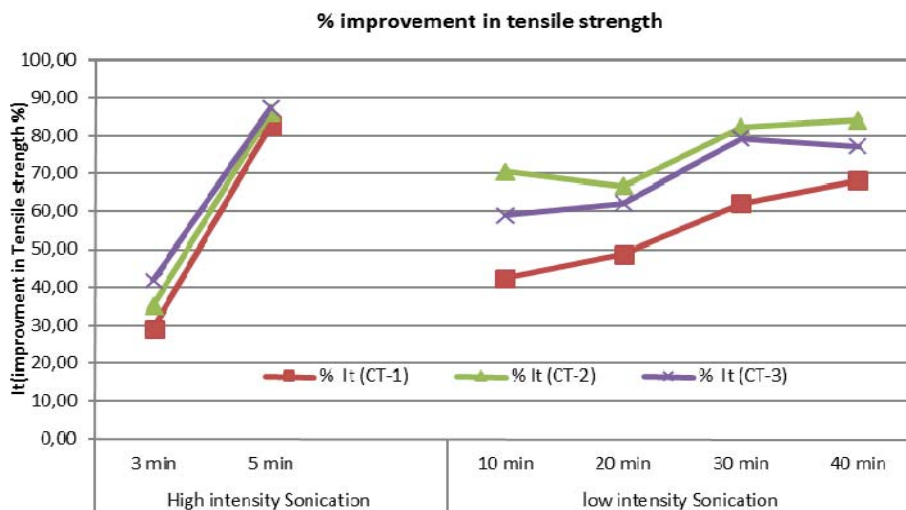
Fig. 7 Relative increase in tensile strength of MWCNTs cementitious composites
