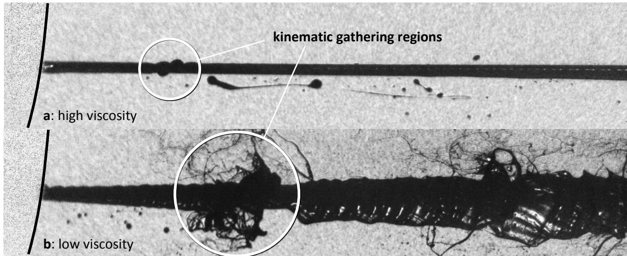
Figure 6: Near-nozzle sprays
