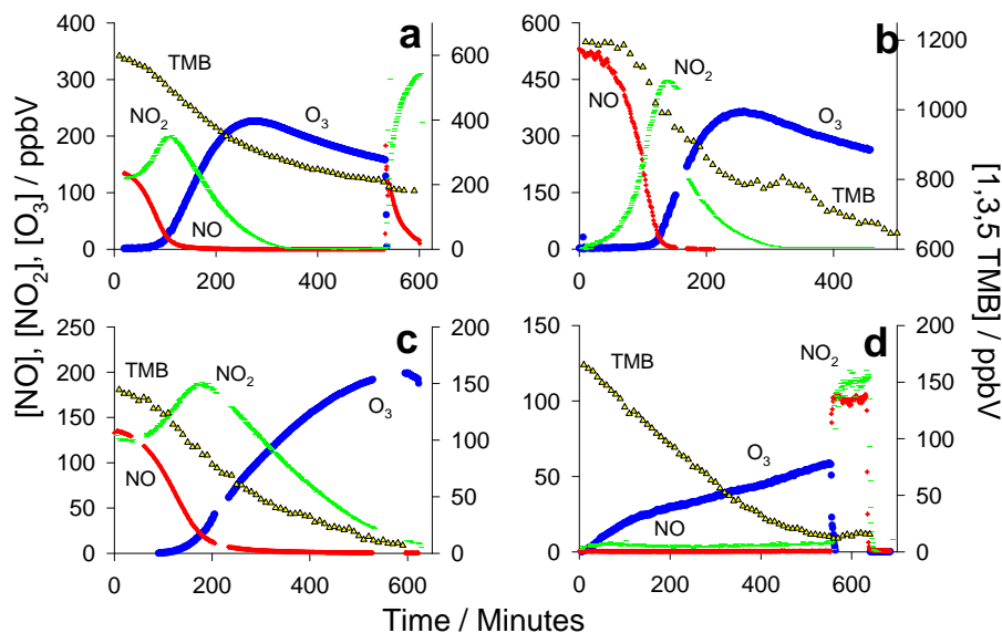
Fig. 1. Temporal evolution of the major gas phase components of the 1,3,5-TMB photooxidation system during (a) Experiment 6 ( \text{VOC}/\text{NO}_x \sim 2:1 ), (b) Experiment 2 ( \text{VOC}/\text{NO}_x \sim 2:1 , NO only), (c) Experiment 3 ( \text{VOC}/\text{NO}_x \sim 1:2 ) and (d) Experiment 7 ( \text{VOC}/\text{NO}_x \sim 17:1 ). In each plot the left ordinate axis gives the concentration of the inorganic components ( \text{NO} , \text{NO}_2 and \text{O}_3 ) while the right axis gives the concentration of TMB.
