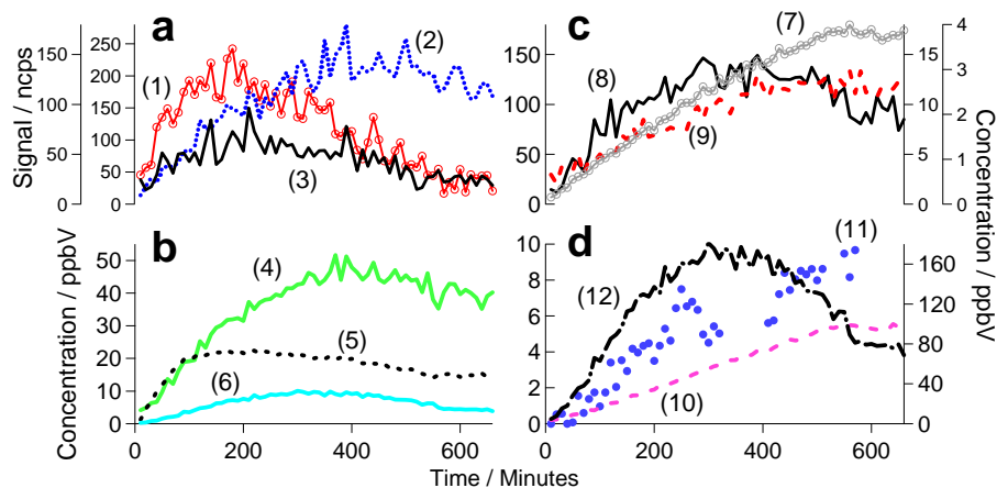
Fig. 10. Temporal evolution of certain key VOCs during the photooxidation of 1,3,5-TMB during experiment 7 ( \text{VOC}/\text{NO}_x \sim 17:1 ). Compound numbering is the same as that used in the caption for Fig. 9. Note: in figure (a) signal of \text{O}_2 -bridged diol (3) is given on the right axis and in figure (d) concentration of hydroxyl acetic acid (10) is given on the left axis.
