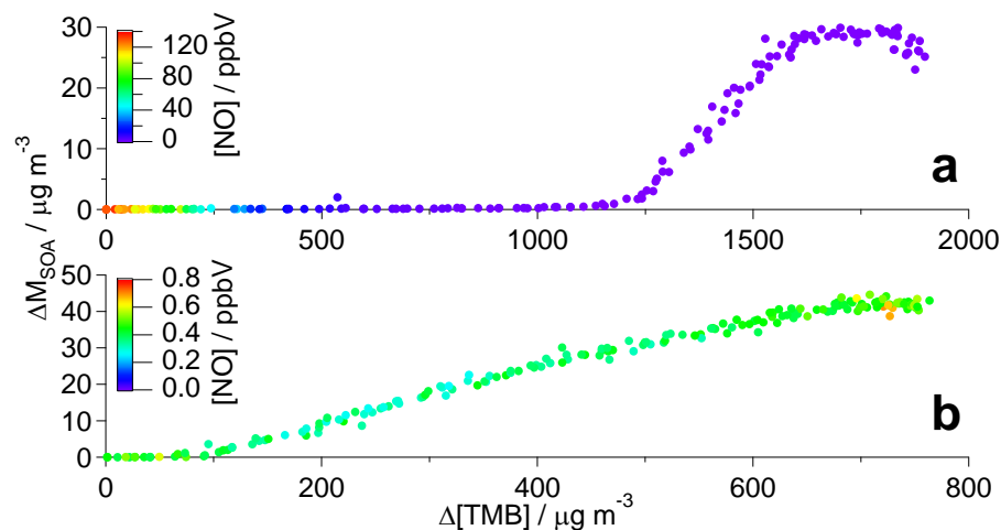
Fig. 5. SOA growth curves for (a) Experiment 6 (high NO x experiment, VOC/NO x ~ 2:1) and (b) Experiment 7 (low NO x experiment, VOC/NO x ~ 17:1). \Delta[\text{TMB}] = reacted mass of TMB following initiation of the oxidation chemistry.
