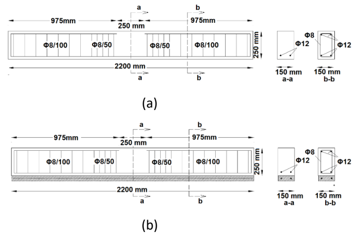
Figure 1. a) Initial and b) Strengthened beams with RC layers
