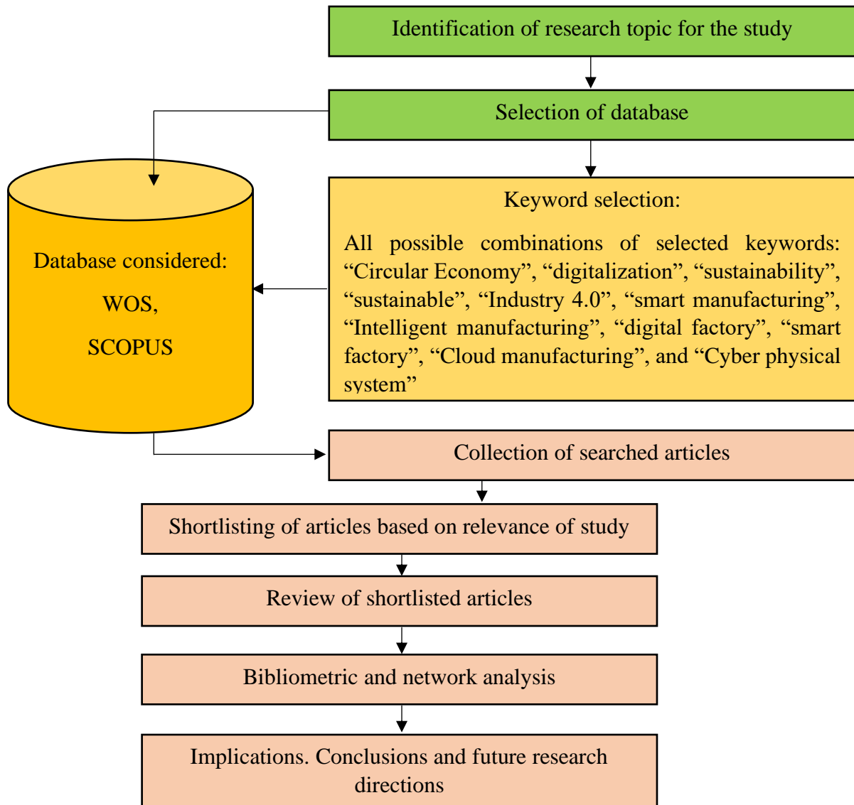
Figure 1. Research methodology
