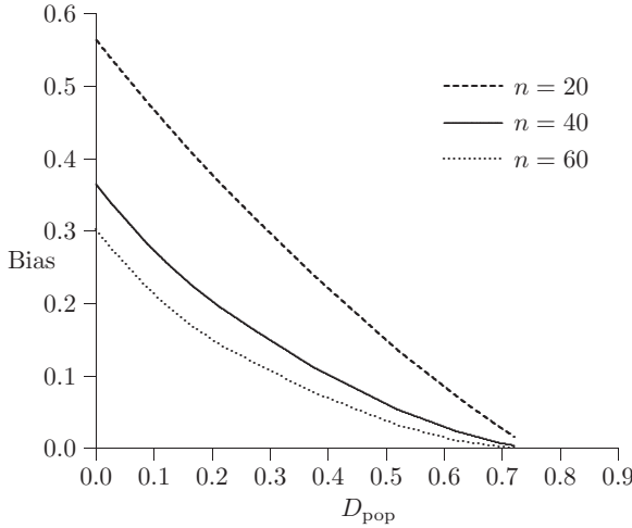
Figure 1. Bias E[D] - D_{pop} , J = 4 , p = 0.1 , equal expected unit sizes.
