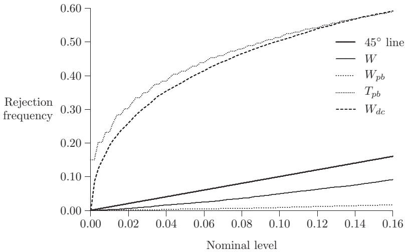
Figure 5. P -value plot, H_0 : D_{pop,1} = D_{pop,1} , power properties.
