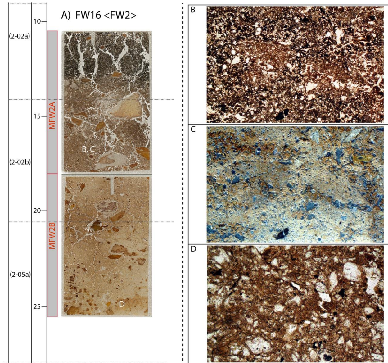
Figure 7: Thin section details from Farley Water FW16 <FW2>, showing: (A) Scan of MFW2A, with contexts (2-02a) and (2-02b). Stony (2-02b) below organic (2-02a) a minerogenic surface peat. Bleached stone rims, caused by hydromorphic (stagnant water) are visible. And (A) Scan of MFW2B, with contexts (2-05a) and (2-02b).. A small relict area of iron-stained argillic brown earth soil is visible (bottom left).
