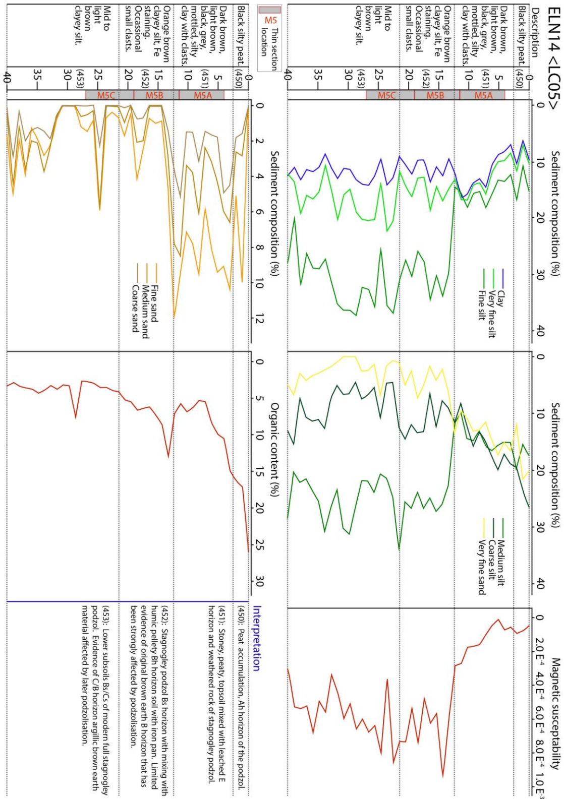
Figure 9: Sediment analysis of sample Lanacombe ELN14 <LC05>.
