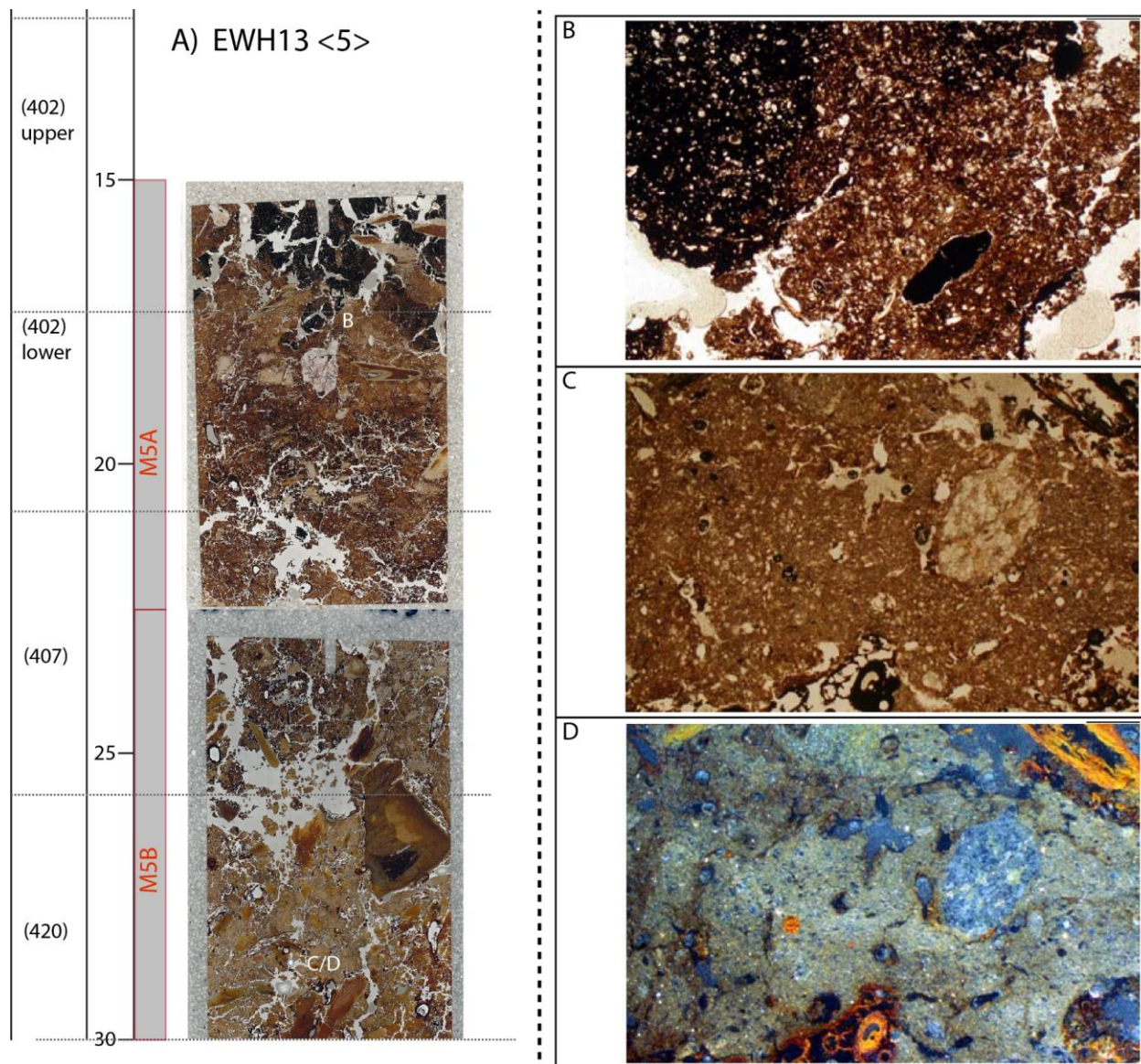
Figure 4: Thin section details from Wintershead EWH13 <5>, showing: (A) Scan of M5A, contexts (402) upper, (402) lower and (407). Scan showing mixed boundary between palaeosol (407) and overlying silty peat (402). Note iron-depleted subsoil containing burnt quartzite. And (A) Scan of M5B, contexts (407) and (420). Scan showing the palaeosol (420) and (407) containing welded soil microfabric/total excremental microfabric).
