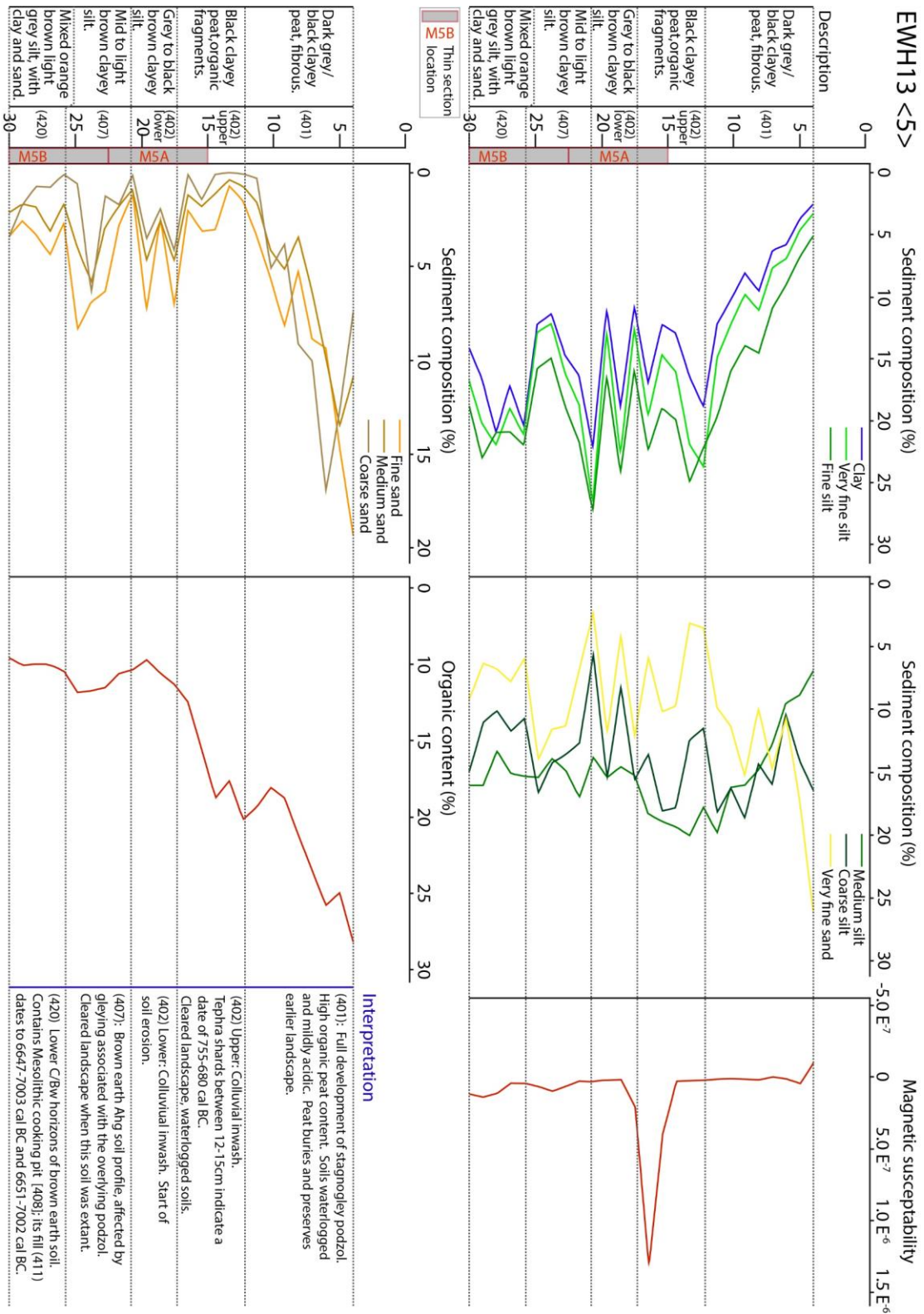
Figure 3: Sediment analysis of sample Wintershead EWH13 <5>.
