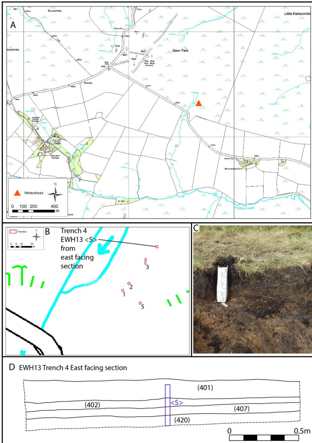
Figure 2: Wintershead EWH13 site investigation showing, A) site location, B) trench 4 relative to the other trenches, C) a working shot of sample EWH13 <5> in the trench section and, D) the east facing section of trench 4.
