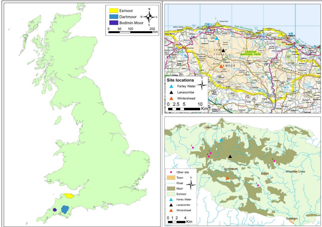
Figure 1: The location of Exmoor National Park at national (A), and regional (B) scales, with the three study sites highlighted and additional sites mentioned in the text (C; 0 = Brightworthy, 1 = Spooners, 2 = Pinkery Canal, 3 = The Chains, 4 = Codsend Moor and 5 = Holworthy hillslope enclosure).
