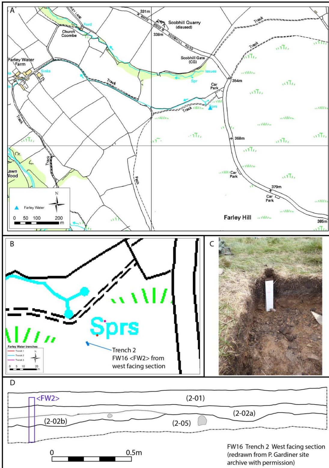
Figure 5: Farley Water FW16 site investigation showing, A) the location of Farley Water (FW16), B) trench 2 relative to the other trenches, C) a working shot of sample FW16 <FW2> in the trench section and, D) the west facing section of trench 2.
