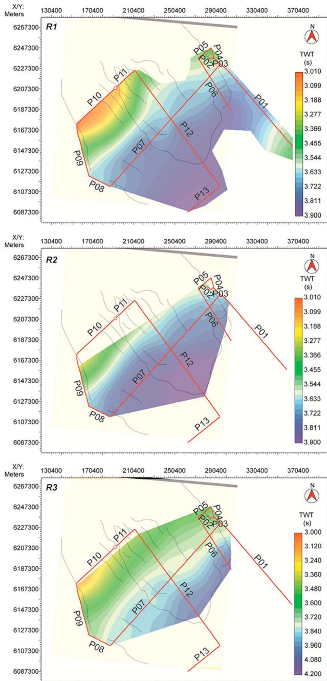
Figure 5. Maps of the three reflectors. Note (a) the widespread distribution of R1 and in (b) the limited distribution of R2 relative to both (a) R1 and (c) R3.
